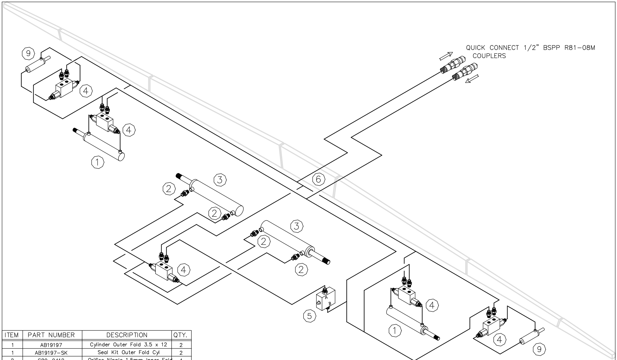
33/36m BOOM STANDARD FOLD OPTION
